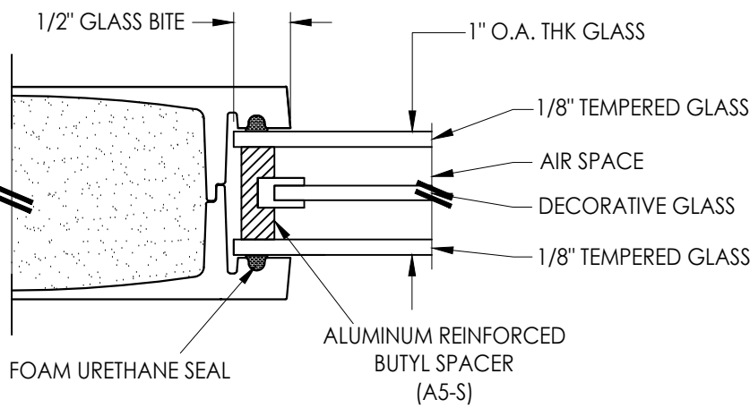
G2 GLAZING DETAIL DECORATIVE GLASS
