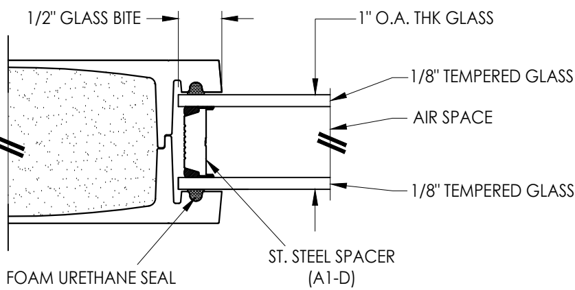
G1 GLAZING DETAIL CLEAR GLASS
