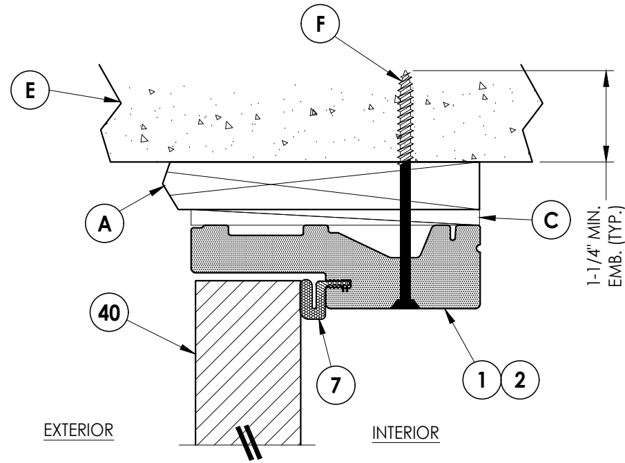
3 VERTICAL CROSS SECTION 5 Outswing Shown (Inswing Similar) Shown w/ 1X Buck
