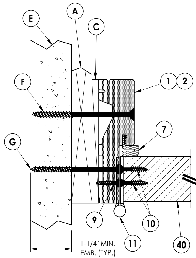
1 HORIZONTAL CROSS SECTION 5 Outswing Shown (Inswing Similar) Shown w/ 1X Buck
